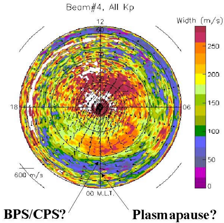
Figure 4: Clock dial contour plot of the statistical average Doppler velocity widths measured on TIGER beam 4 for all values of Kp during December 1999 to February 2000. Otherwise the format of the figure is the same as Figure 3.
