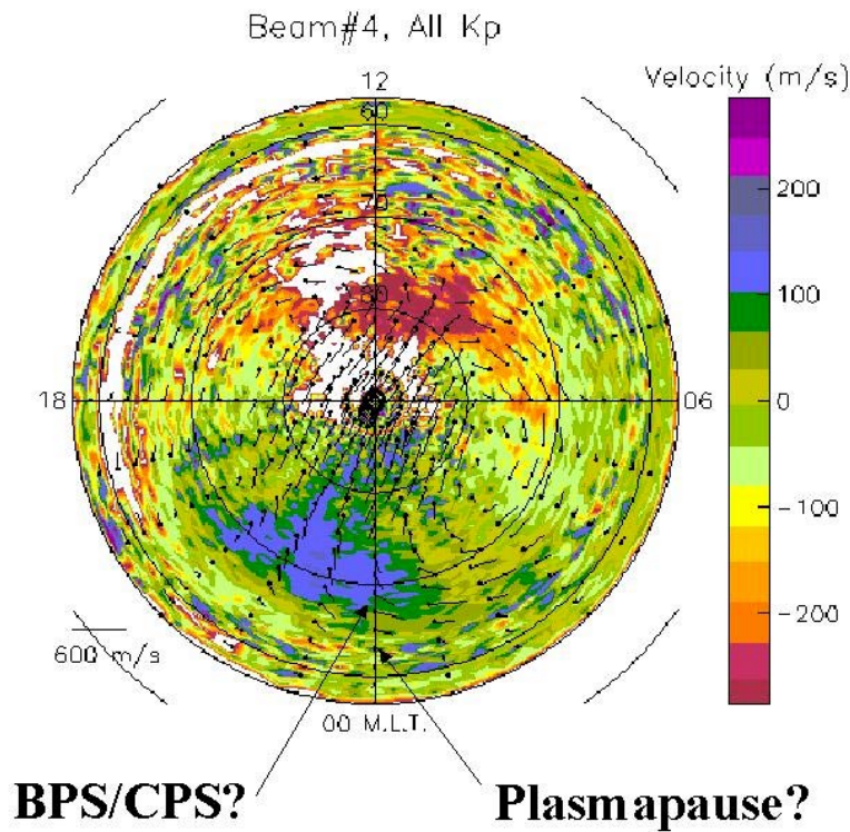
Figure 3: Clock dial contour plot of the statistical average line-of-sight Doppler velocities measured on TIGER beam 4 for all values of Kp during December 1999 to February 2000. An average velocity was calculated for each bin of 15 minutes in magnetic local time (MLT) and each range separated by 45 km. The four black circles superimposed on the plot correspond to AACGM latitudes of 57°, 60°, 70° and 80°S. Probable midnight locations of the boundary between the ionospheric projection of the Boundary Plasma Sheet (BPS) and the Central Plasma Sheet (CPS) (i.e., near the poleward wall of the main ionospheric trough), and the plasmapause, are indicated.
