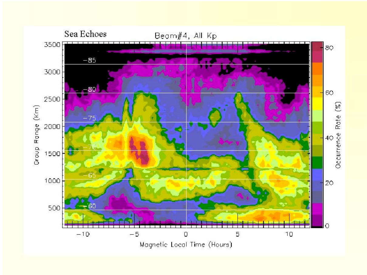
Figure 1: Rectangular contour plot of the occurrence rate of sea echoes detected on TIGER beam 4 for all values of Kp during December 1999 to February 2000. The occurrence rate was calculated for each bin of 15 minutes in magnetic local time (MLT) and each range separated by 45 km. AACGM latitudes are superimposed in white and tick marks on the abscissa are at 30-minute intervals.
