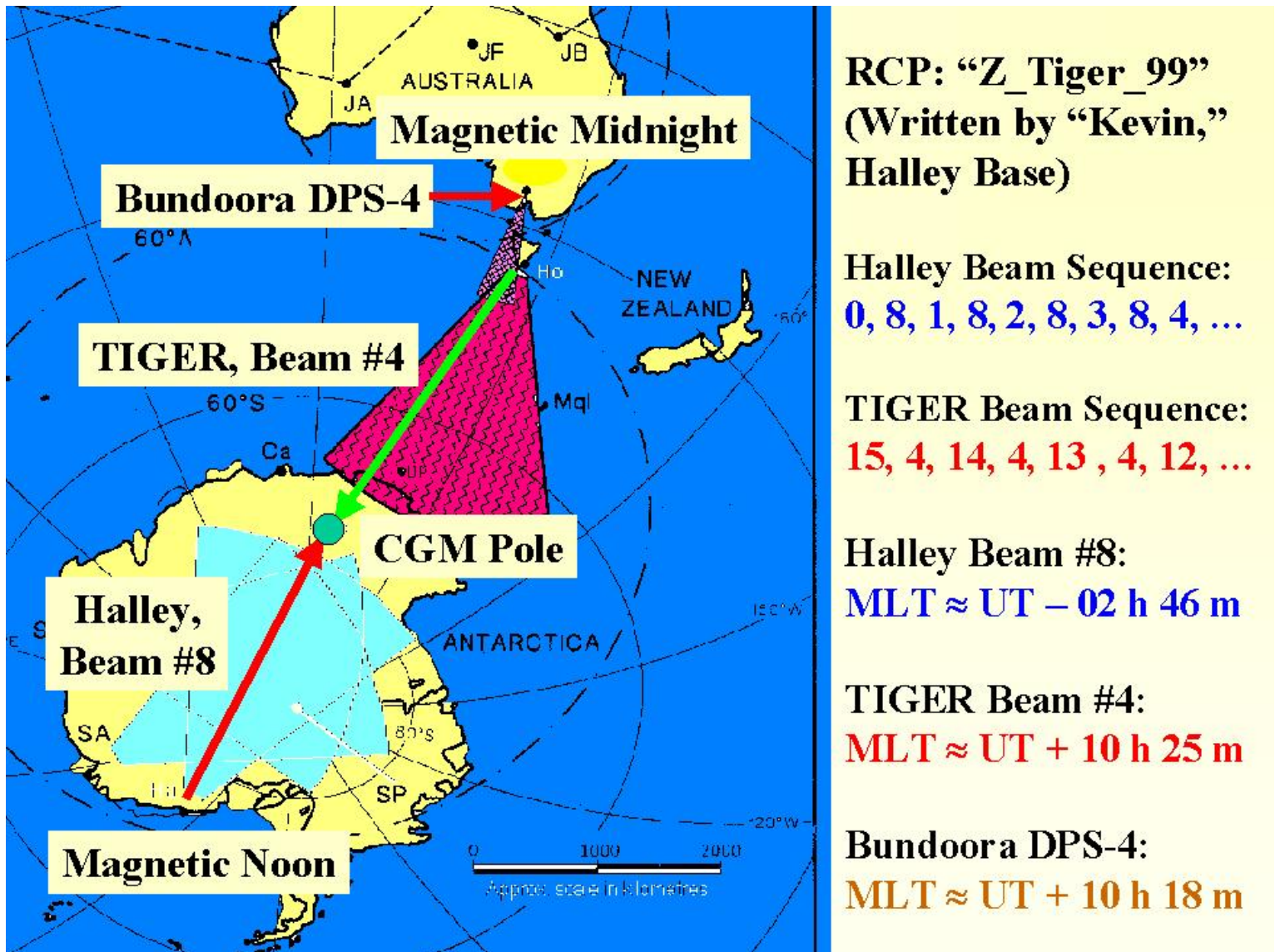
Figure 1: Layout of the experiment designed to measure the time delay between the start of an IMF driven convection change in the dayside ionosphere and its manifestation in the high-latitude nightside ionosphere, and the subsequent penetration of magnetospheric convection fields into the plasmasphere.
