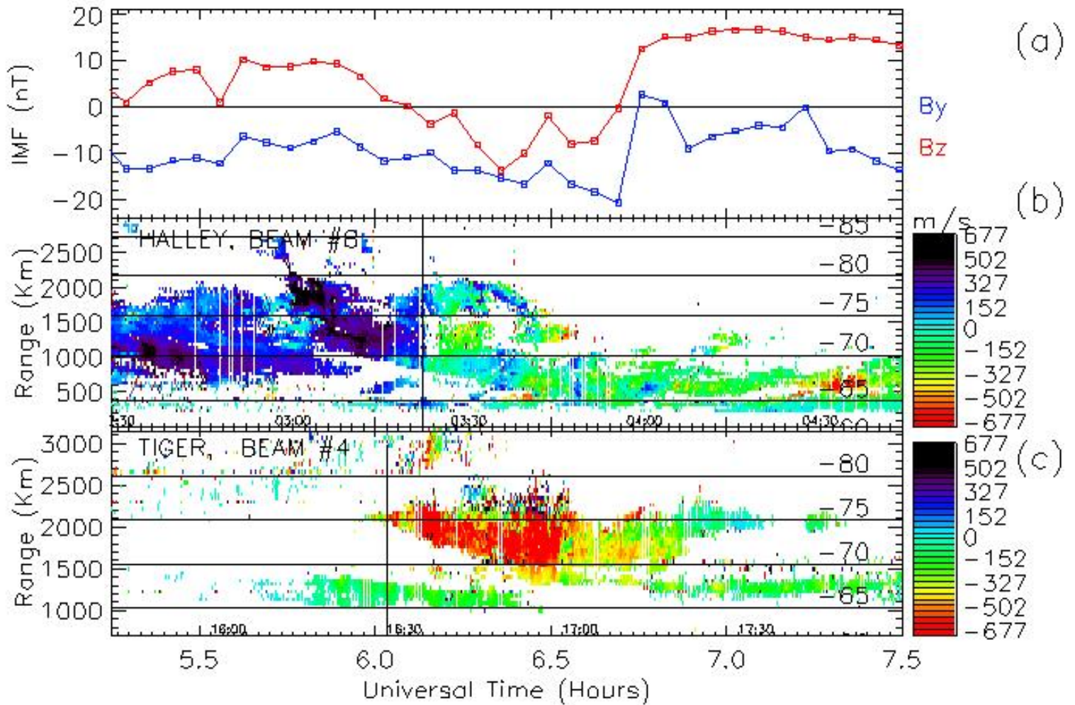
Figure 2: (a) Four-minute averaged values of the B_y (blue) and B_z (red) components of the IMF measured on board the ACE spacecraft during February 12, 2000, 0515 to 0730 UT. The time series was advanced in time to correct for the propagation delay from the spacecraft to the magnetopause, but the correction has a nominal error of 10 minutes. (b) Line-of-sight Doppler velocities for Halley beam 8 for the same time interval as the IMF. (c) Similarly, line-of-sight Doppler velocities for beam 4 of TIGER. The Doppler velocities were color-coded blue to black for approaching velocities and green to red for receding velocities for both radars. The thin vertical white lines are brief outages caused by a bug in an early version of the radar control program. Velocities for sea echoes were rejected and tick marks are at 2-min intervals.
